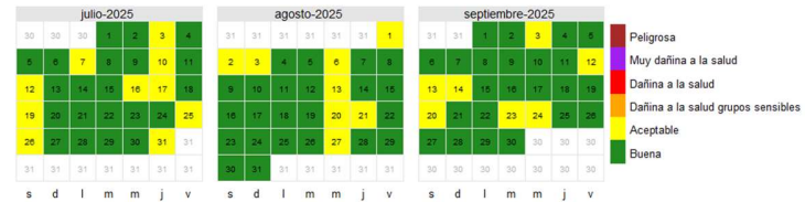
ICA PM 2.5 ECA Yumbo
