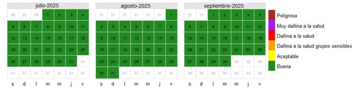
ICA PM 2.5 La Paila
