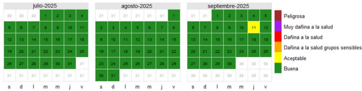
ICA PM 2.5 ECA Cartago
