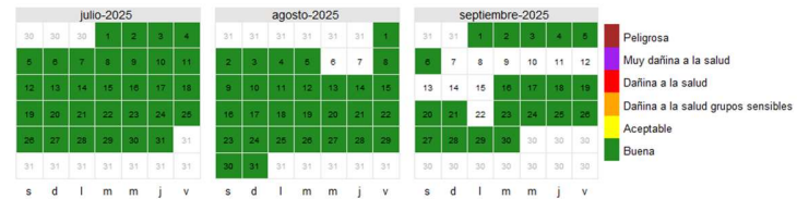
ICA PM 2.5 ECA Buga
