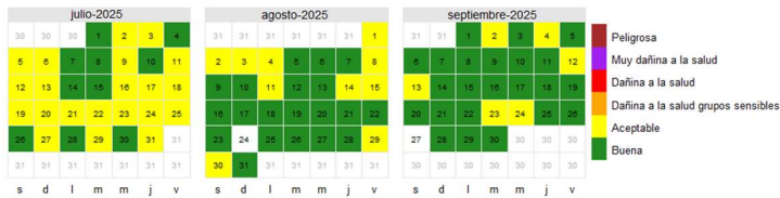
ICA PM 2.5 ECA Tuluá
